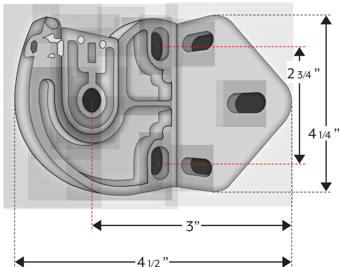
Bracket - (Inside) Side View
